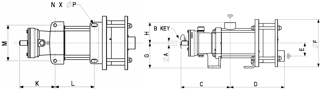
C1-I & C2-I STAINLESS STEEL PUMP DIMENSIONS
