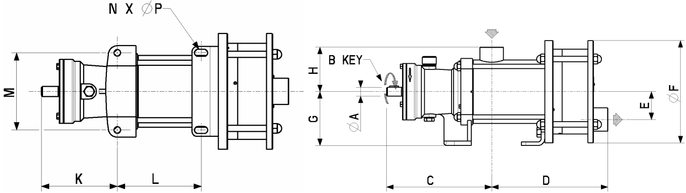
C4-I & C8-I STAINLESS STEEL PUMP DIMENSIONS
